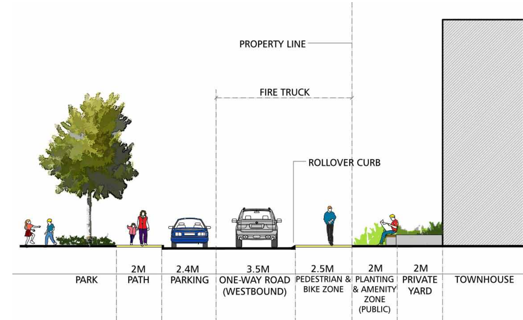
CROSS-SECTION B-B' : NORTH OF PARK AT PARKING CONCEPT 1 SCALE 1:75
