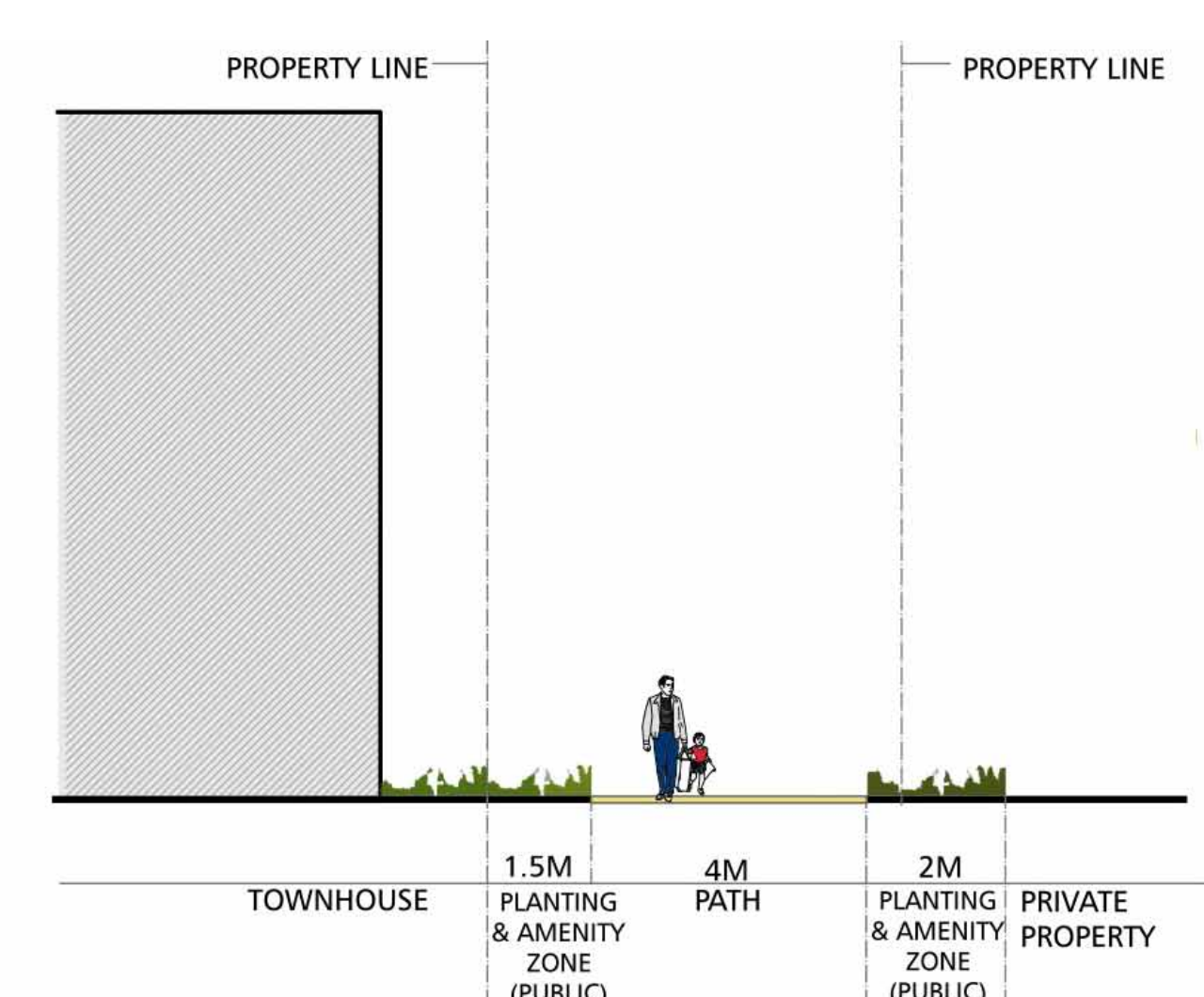
CROSS-SECTION E-E' : NORTH OF PARK CONCEPT 2 SCALE 1:75
