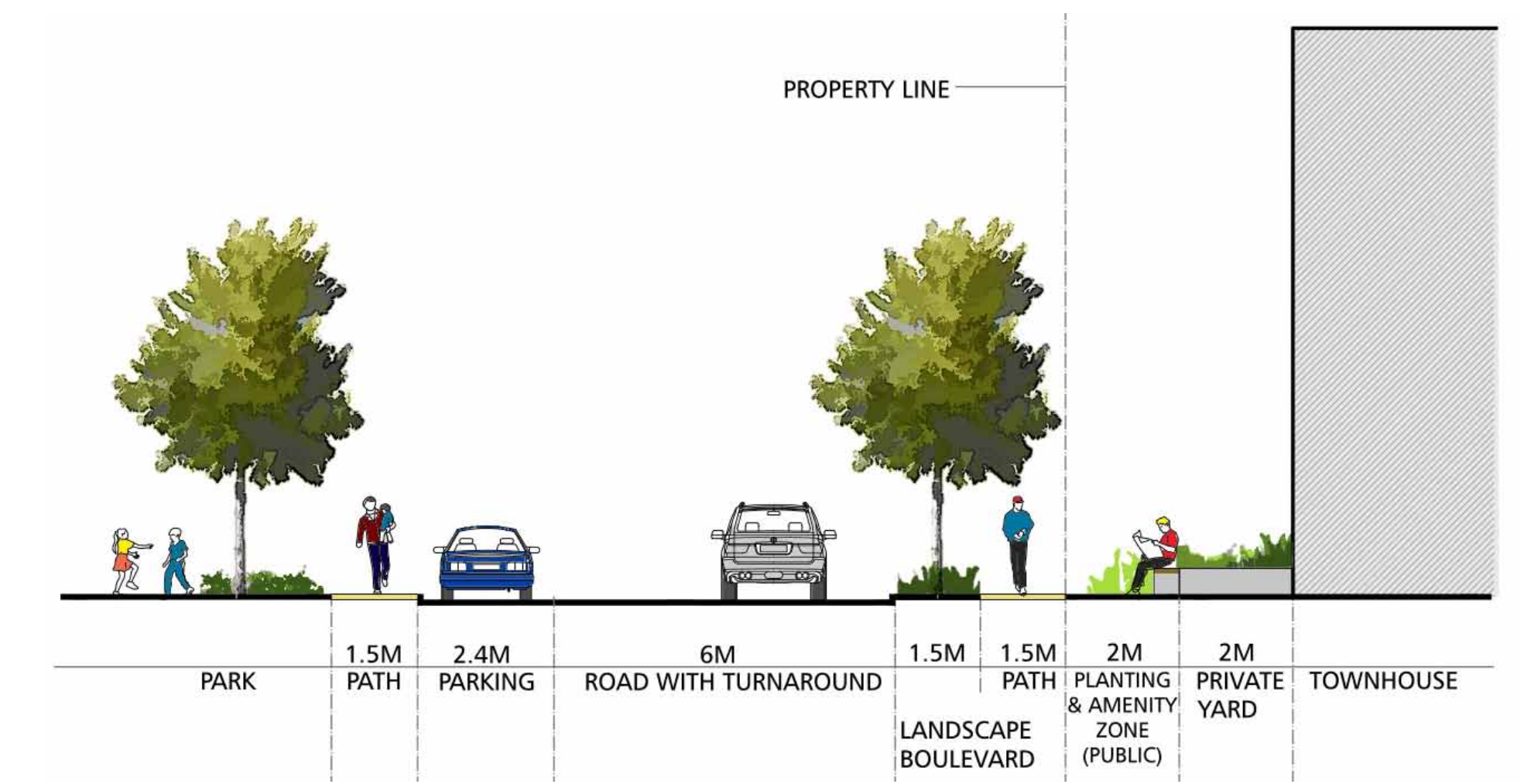
CROSS-SECTION E-E' : NORTH OF PARK CONCEPT 2 SCALE 1:75
