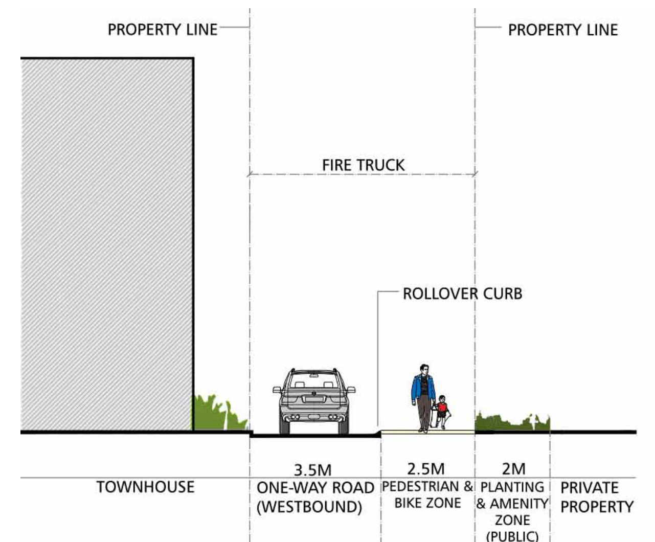
CROSS-SECTION C-C' : NORTH OF PARK CONCEPT 1 SCALE 1:75
