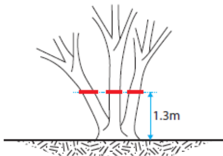
e) Measurement of a multi-stemmed tree*
